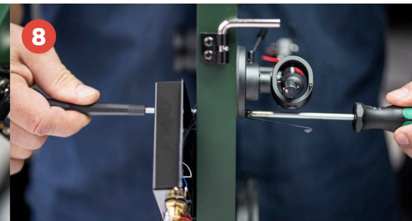
8 Using the PH1 and 5.5mm nut wrench, loosen the tonearm (base) by 3mm.
