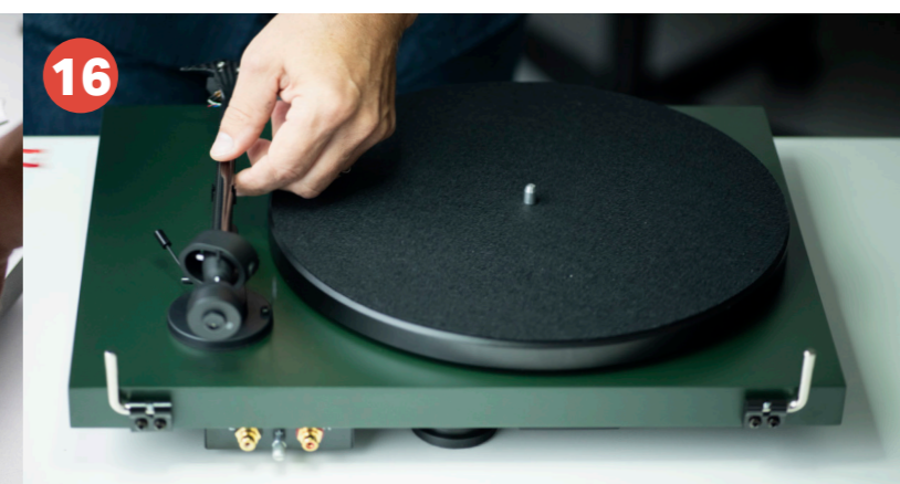
16 Remove the red securing wire and re-install counterweight and anti-skating weight.
