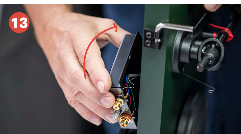
13 Rotate the RCA box back to the initial position.
