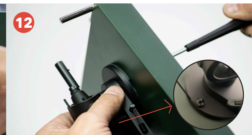
12 Tighten both nuts. Please make sure to hold the antiskating support with your finger while doing so.
