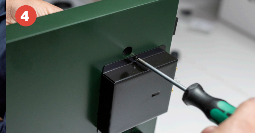
4 Underside: remove upper screw while holding the tonearm from the other side.
