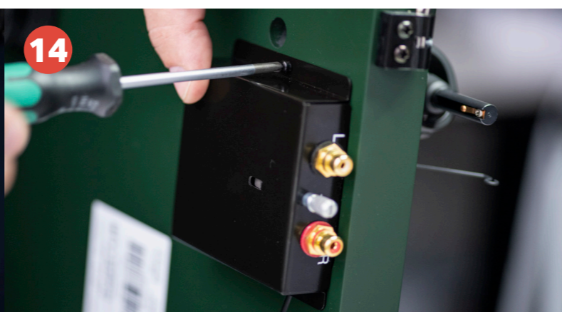
14 Tighten both screws.
