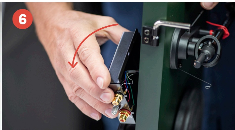
6 Carefully rotate the RCA box...
